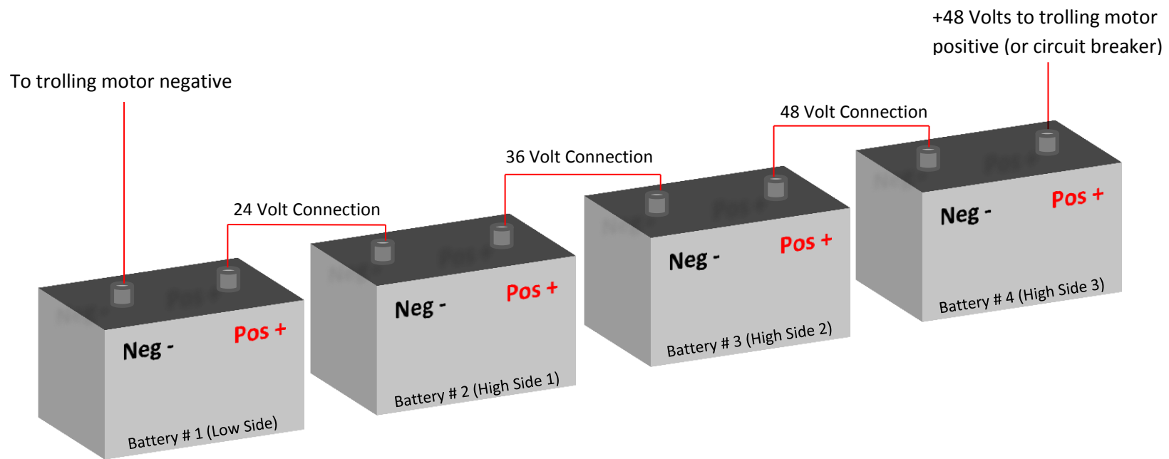
48 Volt Series Connection
