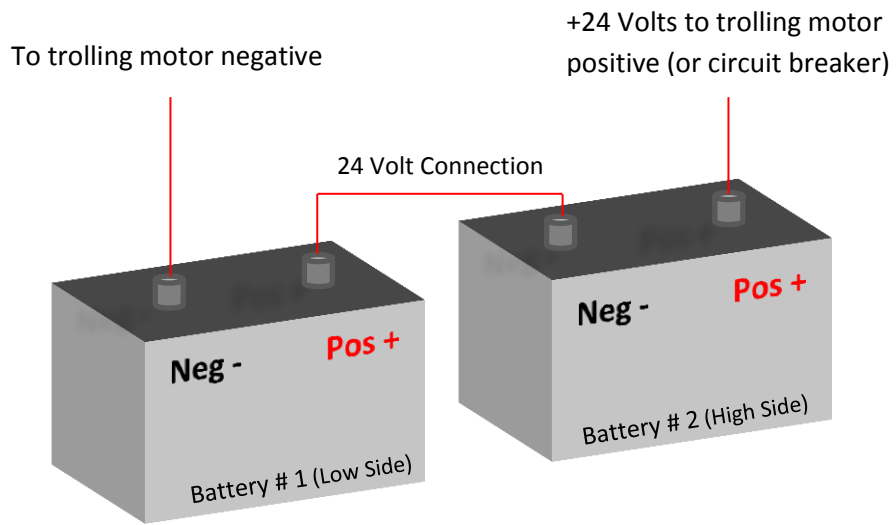
24 Volt Series Connection
