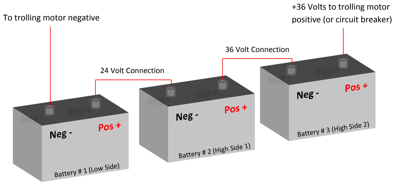
36 Volt Series Connection
